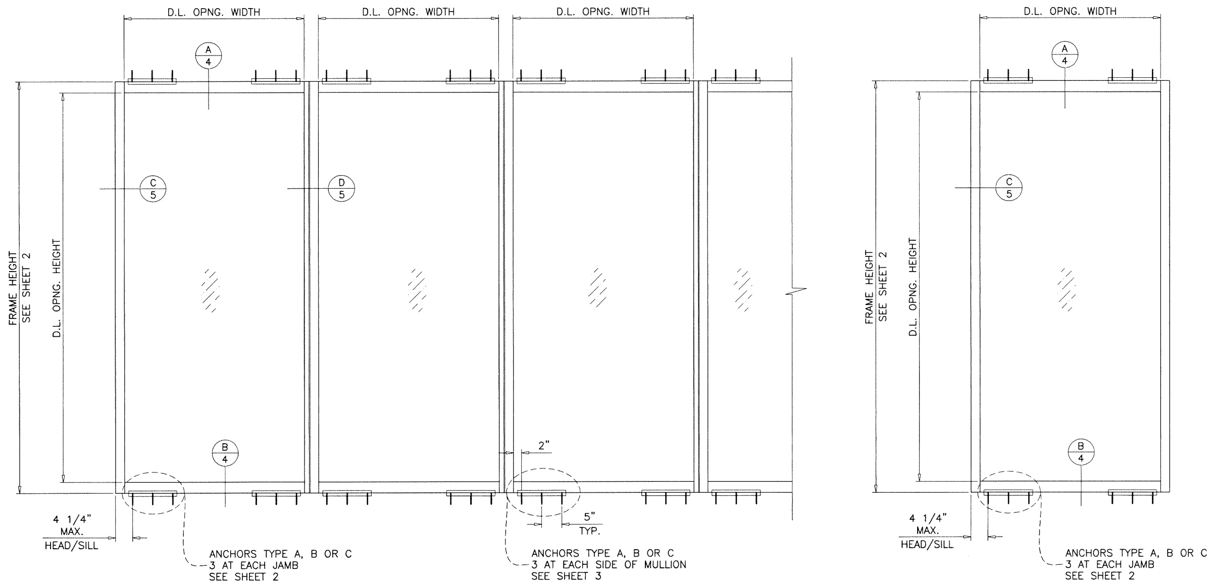
TYPICAL ELEVATIONS
