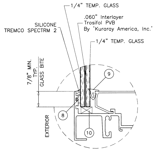
GLAZING DETAIL
